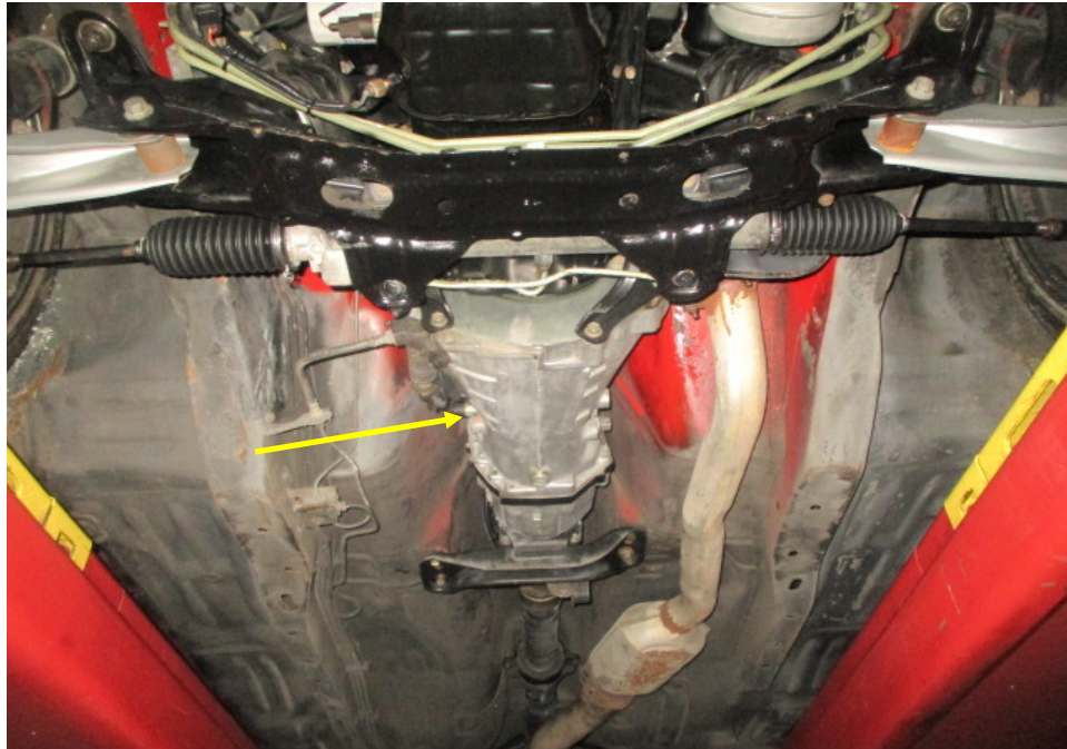
Photo 2 shows a general view of the transmission assembly (arrowed) that was fitted on the Motor Car, as viewed from the front to rear. The front (input) side of the transmission assembly is bolted to the crankshaft side of the engine block while the rear (output) side of the transmission assembly, connects to the propeller shaft, which links to the differential at the rear axle of the Motor Car.
