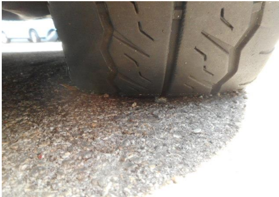
Photo 7 shows the condition of the front right tyre of the Motor Van, which was observed to be in serviceable condition with remaining tread depth of approximately 4.4mm. The tyre, which was wrapped around standard steel wheel rim, was also observed to be sufficiently inflated for vehicular operation. There was no tear, cut or burst mark(s) on the outer and the inner sidewalls as well as across the tread of the 4 tyres that were fitted on the Motor Van.
