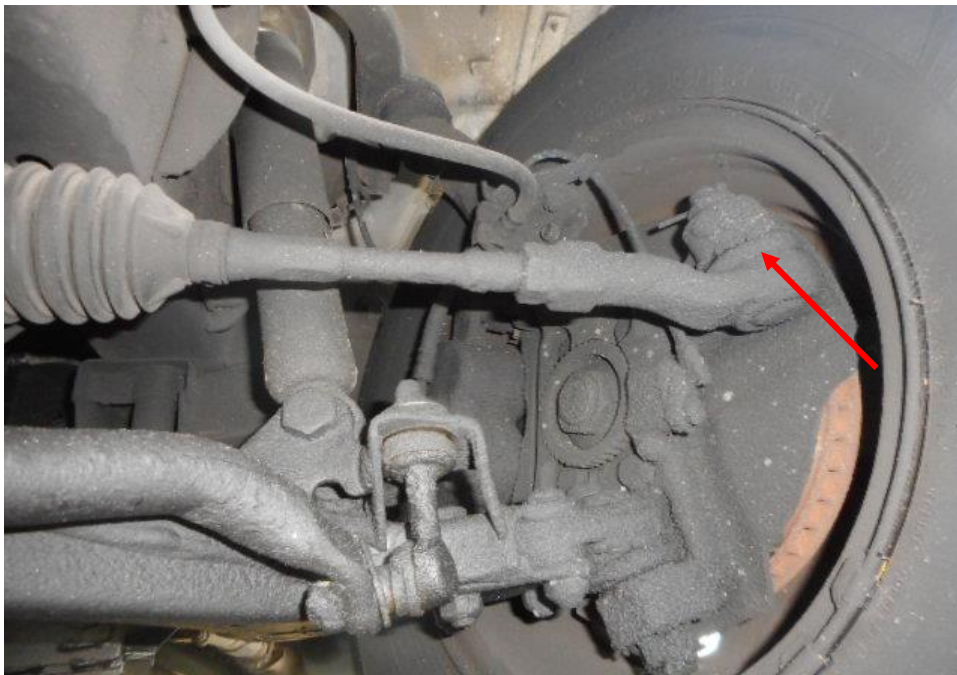
Photo 17 shows the various undercarriage components at the front left wheel of the Motor Van, in particular the steering tie rod end (arrowed). The various undercarriage components of the Motor Van were all found to be intact without any visible damage. There was also no sign of fluid stain(s) observed on the various undercarriage components.
