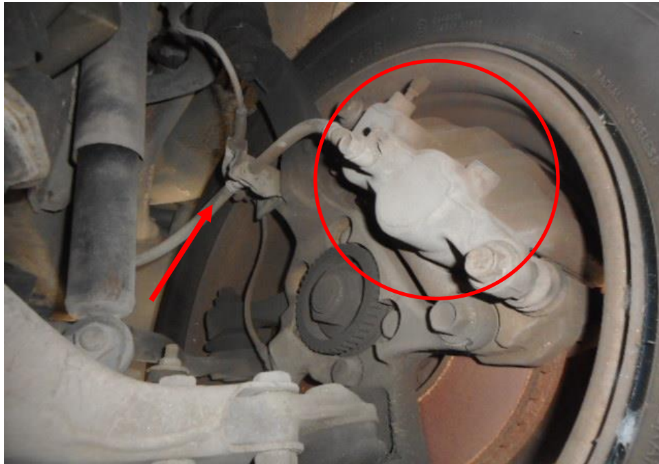
Photo 20 shows the brake hose/pipe (arrowed) at the front right wheel of the Motor Van. No leakage of brake fluid was observed. Visual examination of the various components of the braking system like the brake caliper (circled), brake booster, brake pedal etc had revealed all to be intact and without visible damage at the time of accident. There was also no sign of fluid stain(s) observed on the various undercarriage components.
