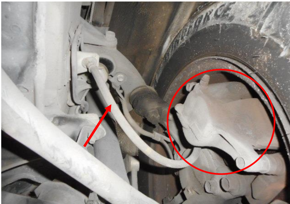
Photo 23 shows the brake hose/pipe (arrowed) at the front right wheel of the Motor Van. No leakage of brake fluid was observed. Visual examination of the various components of the braking system like the brake caliper (circled), brake booster, brake pedal etc had revealed all to be intact and without visible damage at the time of accident. There was also no sign of fluid stain(s) observed on the various undercarriage components.
