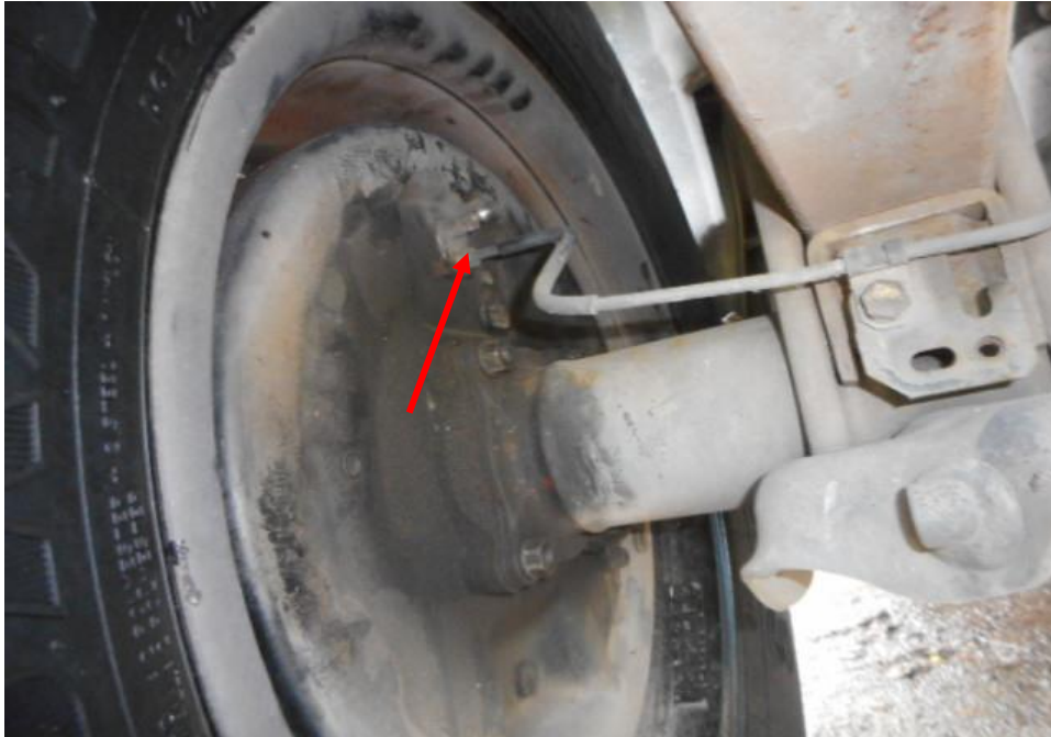
Photo 19 shows the brake pipe (arrowed) at the rear left wheel of the Pick-up truck. I did not observe any leakage of brake fluid at the time of my inspection of the Pick-up truck. My static tests of the Pick-up truck's braking system, along with my visual examination of the various mechanical components in the braking system had indicated that there was no internal leakage of pressure/vacuum. Hence the braking system of the Pick-up truck was likely to be in serviceable condition at the material time of accident.
