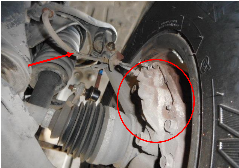
Photo 20 shows the brake hose/pipe (arrowed) at the front right wheel of the Pick-up truck. No leakage of brake fluid was observed. Visual examination of the various components of the braking system like the brake caliper (circled), brake booster, brake pedal etc had revealed all to be intact and without visible damage at the time of accident. There was also no sign of fluid stain(s) observed on the various undercarriage components.
