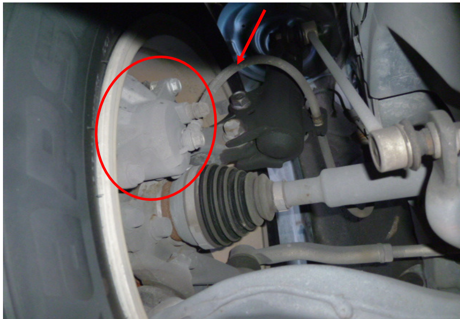
Photo 17 shows the brake hose/pipe (arrowed) at the front right wheel of the Motor Car. No leakage of brake fluid was observed. Visual examination of the various components of the braking system like the brake caliper (circled), brake pedal etc. had revealed all to be intact and without visible damage.
