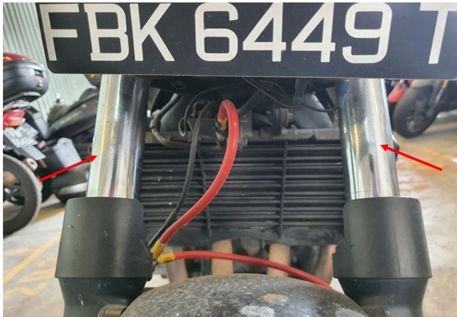
Photo 20 shows the front forks (arrowed) of the Motorcycle. The front forks and fork bracket of the Motorcycle were both found to be intact and undamaged. Turning the Motorcycle's handle bar towards the left and right did not produce any abnormal free play and/or resistance. The steering system of the Motorcycle was in serviceable condition at the time of our inspection.
