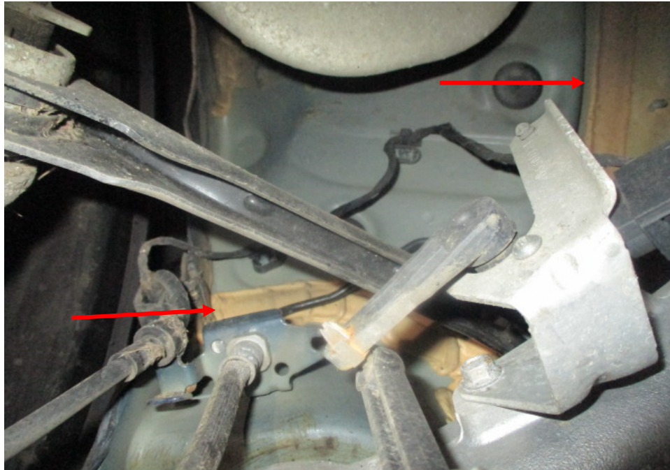
Photo 28 shows the chassis/structural body at the underside rear left of the Motor Car. I did not find any weld marks other than original spot weld marks on the chassis/structural body of the Motor Car. The original factory sealant (arrowed) at the joints along the chassis/structural body was untouched, indicating no work was done on the chassis/structural body of the Motor Car and that the chassis/structural body was originally fitted.
