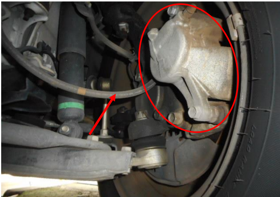
Photo 21 shows the brake hose/pipe (arrowed) at the front right wheel of the Motor Van. No leakage of brake fluid was observed. Visual examination of the various components of the braking system like the brake caliper (circled), brake booster, brake pedal etc had revealed all to be intact and without visible damage at the time of accident. There was also no sign of fluid stain(s) observed on the various undercarriage components.
