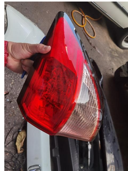
32/44: Taillamp RH - Studs Cracked
