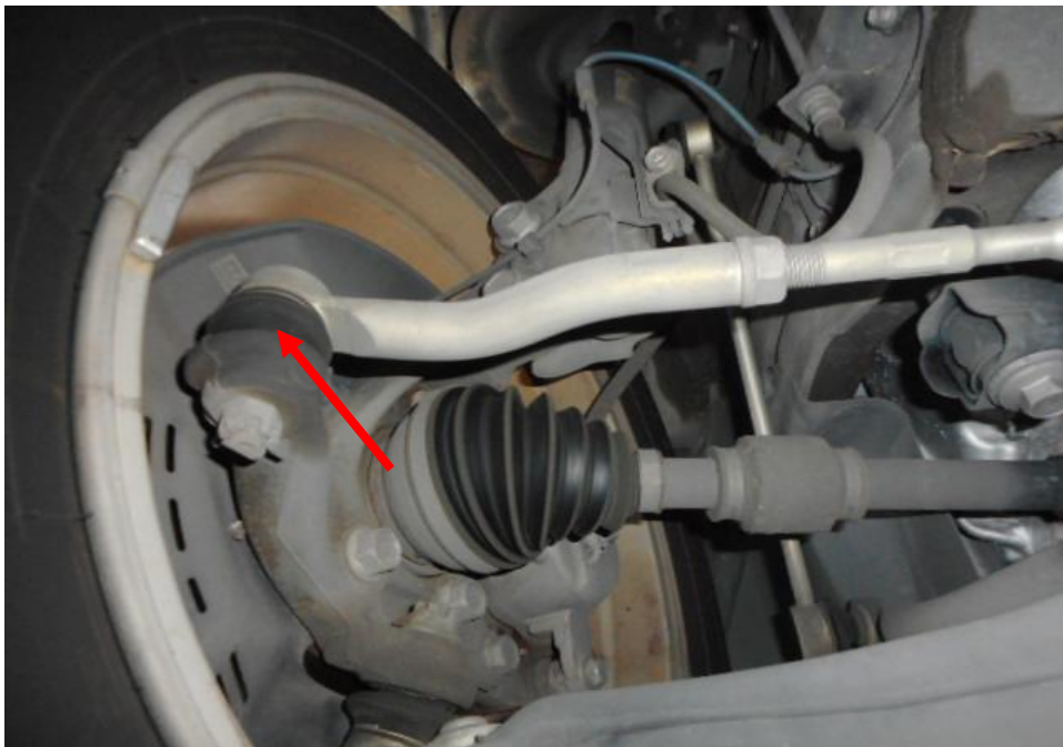
Photo 21 shows the various undercarriage components at the front left wheel of the Motor Taxi, which had included the steering tie rod (arrowed). The various undercarriage components of the Motor Taxi were all found to be intact without any visible damage.
