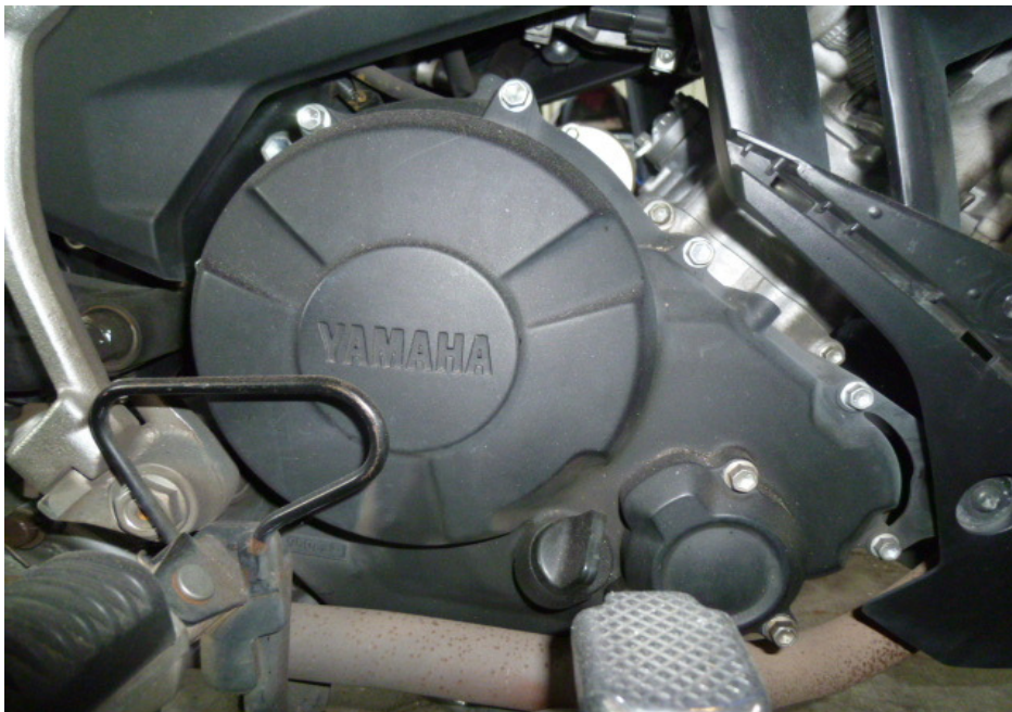
Photo 20 shows the right side of the engine of the Motorcycle at the time of our inspection. The various engine related parts and components were found to be intact with no visible damage. There was also no sign(s) or indication(s) of fluid leak observed around the right engine area of the Motorcycle.
