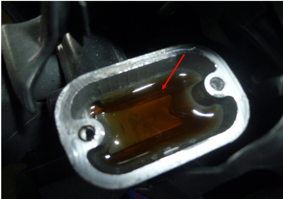
Photo 27 shows the brake fluid reservoir for the front brake of the Motorcycle. The brake fluid was observed to be of sufficient level for operating purposes. However it was found to be slightly contaminated (arrowed).
