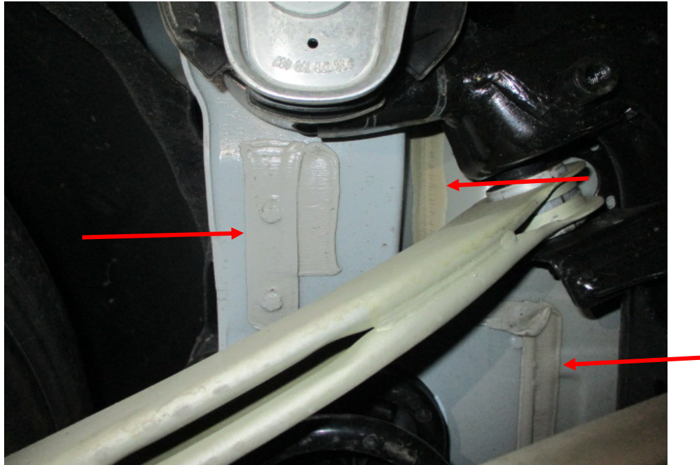
Photo 26 shows the chassis/structural body at the underside rear left of the Motor Car. I did not find any weld marks other than original spot weld marks on the chassis/structural body of the Motor Car. The original factory sealant (arrowed) at the joints along the chassis/structural body was untouched, indicating no work was done on the chassis/structural body of the Motor Car and that the chassis/structural body was originally fitted.
