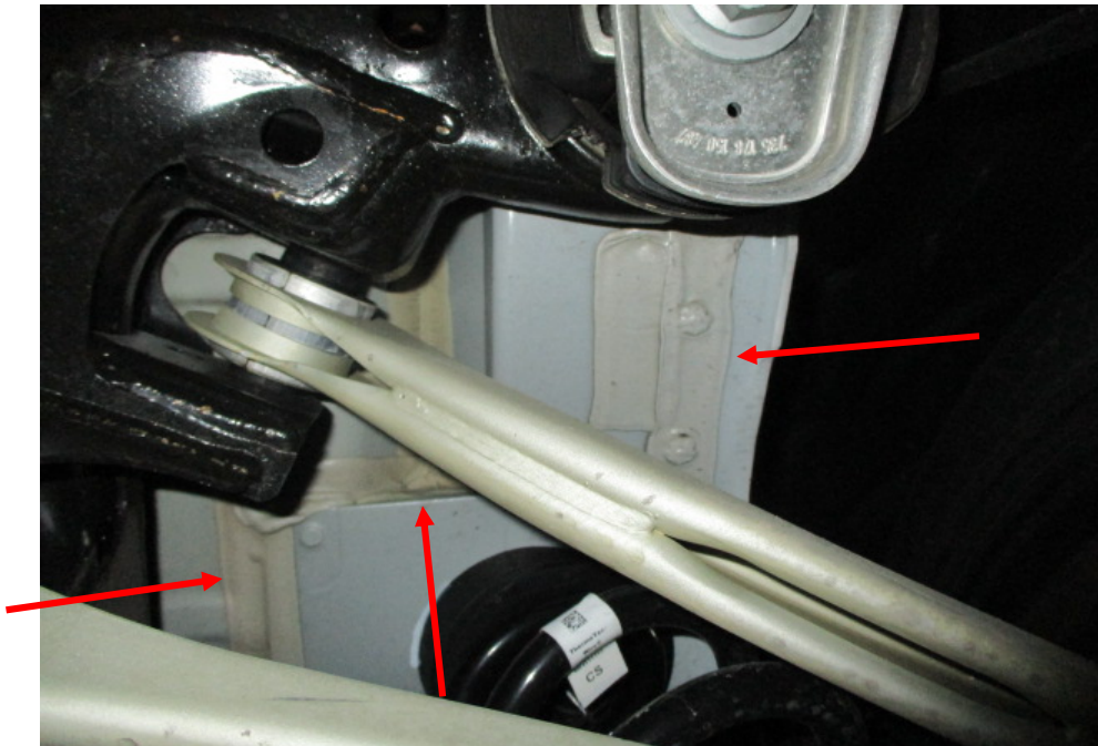
Photo 25 shows the chassis/structural body at the underside rear right of the Motor Car. I did not find any weld marks other than original spot weld marks on the chassis/structural body of the Motor Car. The original factory sealant (arrowed) at the joints along the chassis/structural body was untouched, indicating no work was done on the chassis/structural body of the Motor Car and that the chassis/structural body was originally fitted.
