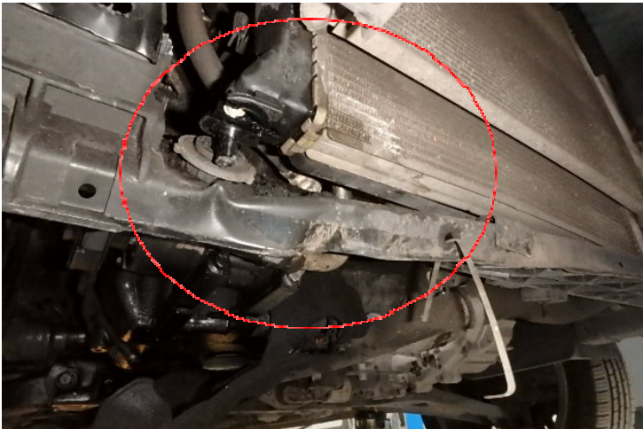
front support panel & radiator assy – merimen photo no. 6/18
