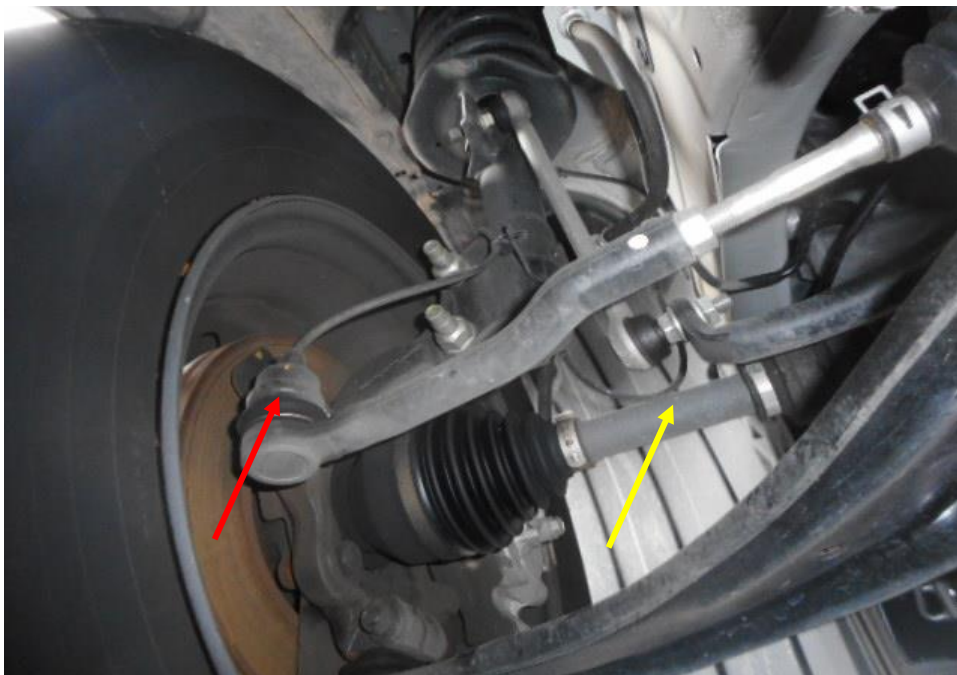
Photo 17 shows the various undercarriage components at the front left wheel of the Motor Van, in particular the steering tie rod end (red arrow) and the driveshaft (yellow arrow). The various undercarriage components of the Motor Van were all found to be intact without any visible damage. There was also no sign of fluid stain(s) observed on the various undercarriage components.
