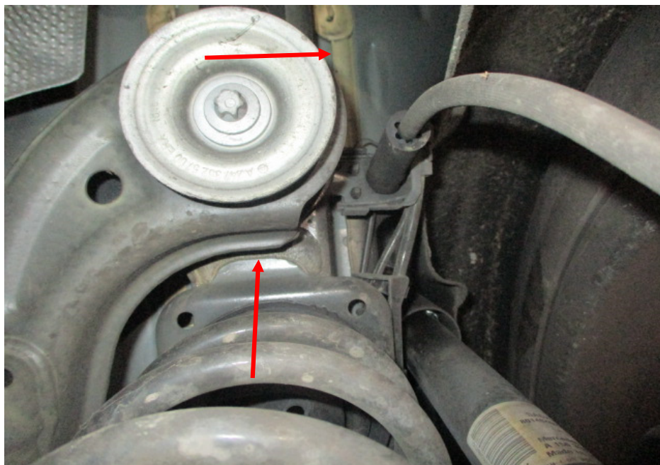
Photo 24 shows the chassis/structural body at the underside rear right of the Motor Car. I did not find any weld marks other than original spot weld marks on the chassis/structural body of the Motor Car. The original factory sealant (arrowed) at the joints along the chassis/structural body was untouched, indicating no work was done on the chassis/structural body of the Motor Car and that the chassis/structural body was originally fitted.
