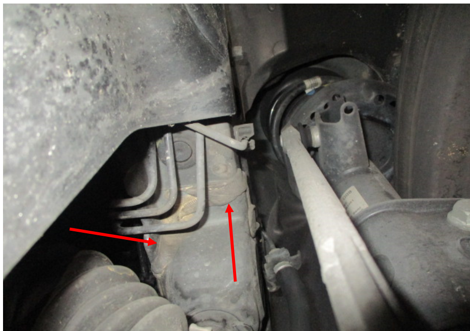
Photo 26 shows the chassis/structural body at the underside front left of the Motor Car. I did not find any weld marks other than original spot weld marks on the chassis/structural body of the Motor Car. The original factory sealant (arrowed) at the joints along the chassis/structural body was untouched, indicating no work was done on the chassis/structural body of the Motor Car and that the chassis/structural body was originally fitted.
