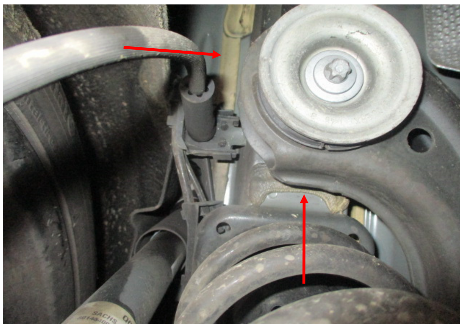
Photo 25 shows the chassis/structural body at the underside rear left of the Motor Car. The original factory sealant (arrowed) at the joints along the chassis/structural body was observed to be untouched. In general, I had found no work was carried out on the chassis/structural body of the Motor Car. The chassis/structural body of the Motor Car was originally fitted.
