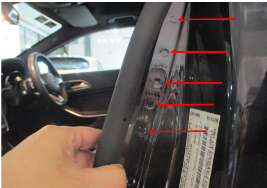
Photo 28 shows the left side "B" pillar of the Motor Car. I did not find any weld marks other than original spot weld marks (arrowed) on the left side "B" pillar of the Motor Car which, indicates that there was no re-welding works carried out. In general, I had found all the non-detachable body panels of the Motor Car to be originally fitted at the time of my inspection.
