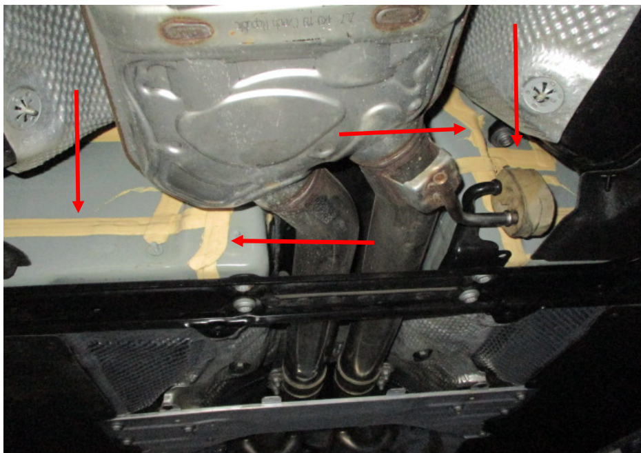
Photo 30 shows the floorboard at the underside centre of the Motor Car. The original factory sealant (arrowed) at the joints along the floorboard was observed to be untouched. In general, I had found all the non-detachable body panels of the Motor Car to be originally fitted at the time of my inspection
