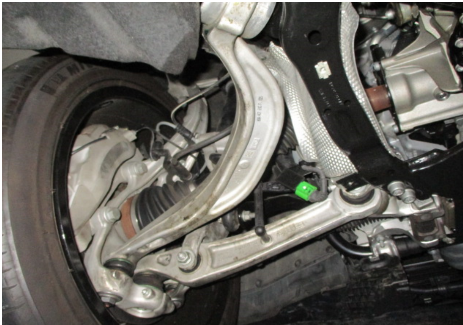
Photo 23 shows the various undercarriage components at the front left wheel of the Motor Car. The mechanical components, control arms and linkages were all found to be intact and secured in an appropriate manner. I also did not observe any fluid leak and/or fluid stain on the underside of the Motor Car.
