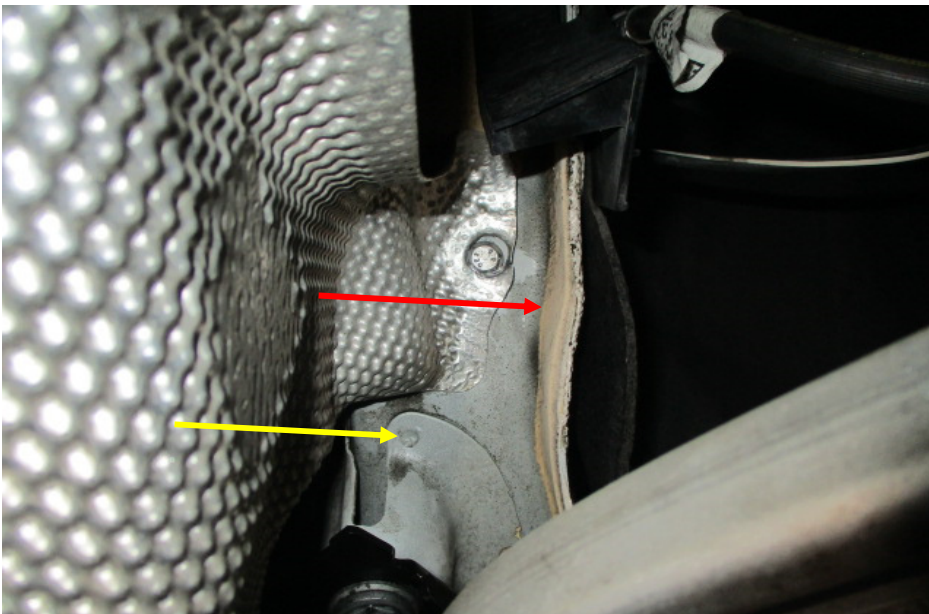
Photo 29 shows the chassis/structural body at the underside front left of the Motor Car. I did not find any weld marks other than original spot weld marks (yellow arrow) on the chassis/structural body of the Motor Car. The original factory sealant (red arrow) at the joints along the chassis/structural body was untouched, indicating no work was done on the chassis/structural body of the Motor Car and that the chassis/structural body was originally fitted.
