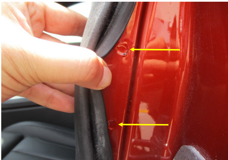
Photo 32 shows the left side "B" pillar of the Motor Car. I did not find any weld marks other than original spot weld marks (arrowed) on the left side "B" pillar of the Motor Car which, indicates that there was no re-welding works carried out. In general, I had found all the non-detachable body panels of the Motor Car to be originally fitted at the time of my inspection.
