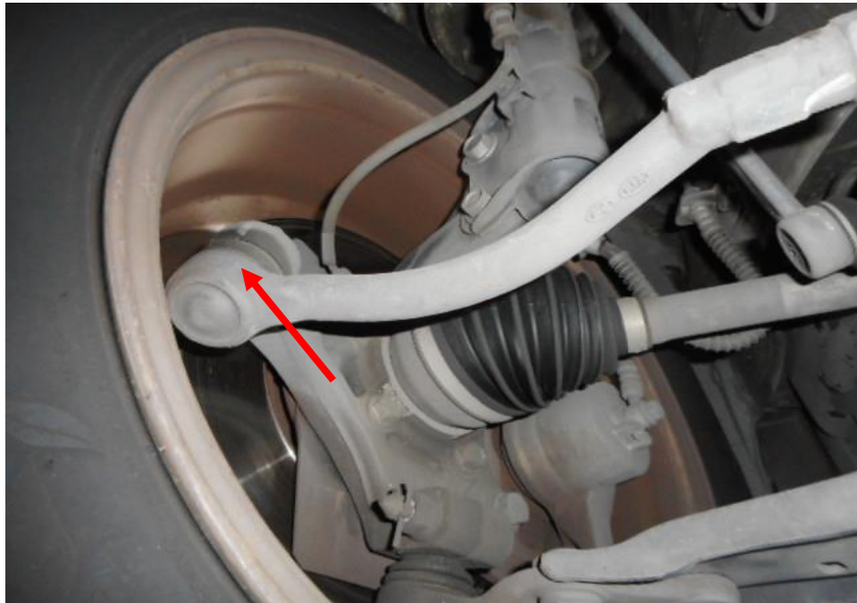
Photo 22 shows the various undercarriage components at the front left wheel of the Motor Taxi, which had included the steering tie rod (red arrow). The various undercarriage components of the Motor Taxi were all found to be intact without any visible damage.
