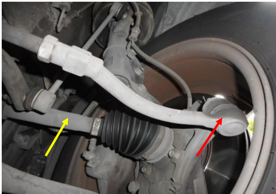
Photo 21 shows the various undercarriage components at the front right wheel of the Motor Taxi, in particular the steering tie rod (red arrow) and drive shaft (yellow arrow). The various steering components were all found to be intact, suggesting that the steering system of the Motor Taxi was likely to be in serviceable condition at the material time of accident. There was also no sign of fluid stain observed on the various undercarriage components at the front right wheel of the Motor Taxi.
