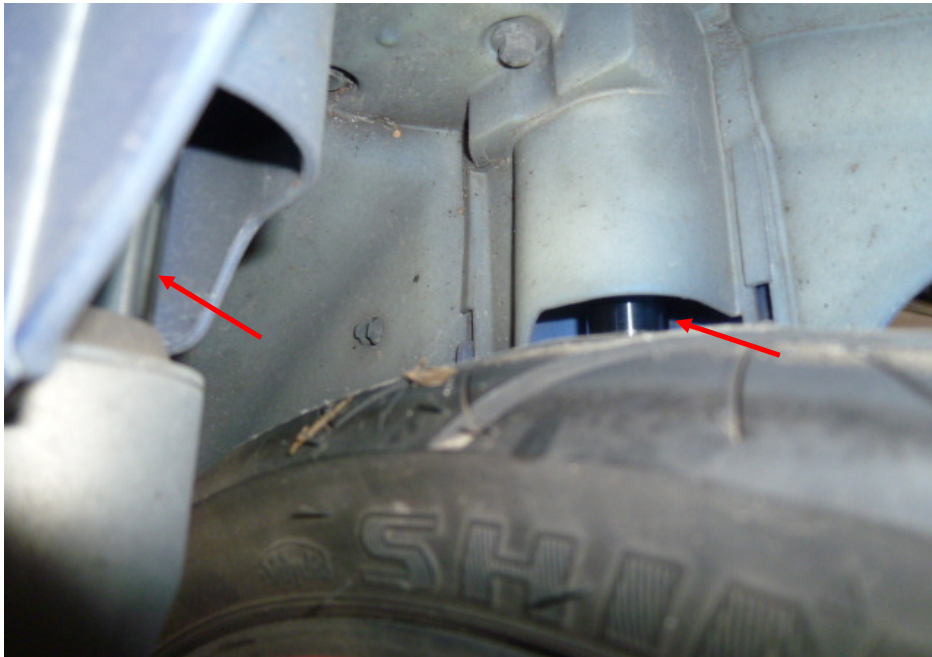
Photo 19 shows the front fork (arrowed) of the Motorcycle. Its front fork was found to be intact. Turning the handle bar towards the right did not produce any abnormal free play and/or resistance. However we were unable to turn the handle bar towards the left due to resistance most probably as a result of damages sustained during the accident.
