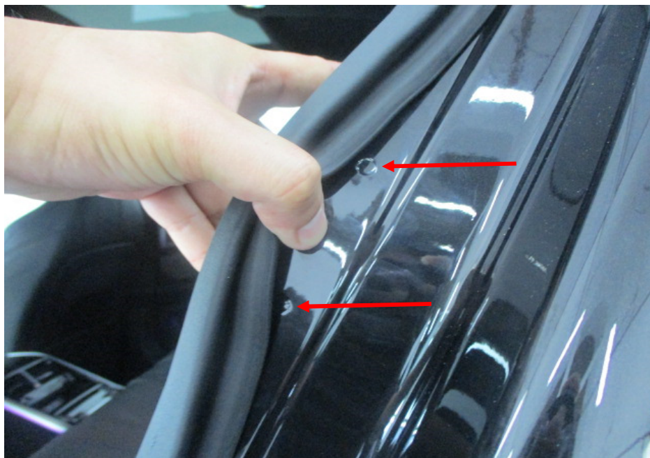
Photo 34 shows the left side "C" pillar of the Motor Car. I did not find any weld marks other than original spot weld marks (arrowed) on the left side "C" pillar of the Motor Car which, indicates that there was no re-welding works carried out. In general, I had found all the non-detachable body panels of the Motor Car to be originally fitted at the time of my inspection.
