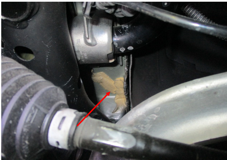
Photo 24 shows the chassis/structural body at the underside front left of the Motor Car. The original factory sealant (arrowed) at the joints along the chassis/structural body was observed to be untouched. In general, I had found no work was carried out on the chassis/structural body of the Motor Car. The chassis/structural body of the Motor Ca was originally fitted.
