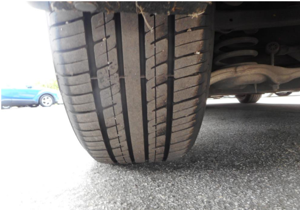
Photo 9 shows the condition of the rear left tyre of the Motor Taxi, which was observed to be in serviceable condition with remaining tread depth of approximately 6.3mm. The tyre, which was wrapped around steel wheel rim, was also observed to be sufficiently inflated for vehicular operation. The 4 tyres of the Motor Taxi were wrapped around standard steel wheel rims.
