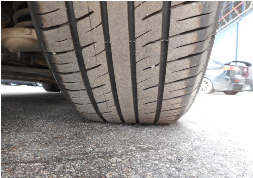
Photo 8 shows the condition of the rear right tyre of the Motor Taxi, which was observed to be in serviceable condition with remaining tread depth of approximately 4.3mm. The tyre was also observed to be sufficiently inflated for vehicular operation with no tear, cut or burst mark(s).
