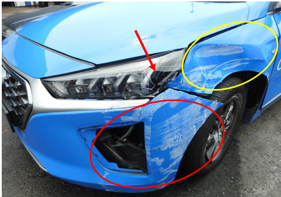
Photo 3 shows the close up view of the Motor Car's front body at the time of my inspection. The Motor Car was observed to have sustained damage at its front left headlamp (arrowed), front bumper (red circle) and front left fender (yellow circle), as a result of the accident.
