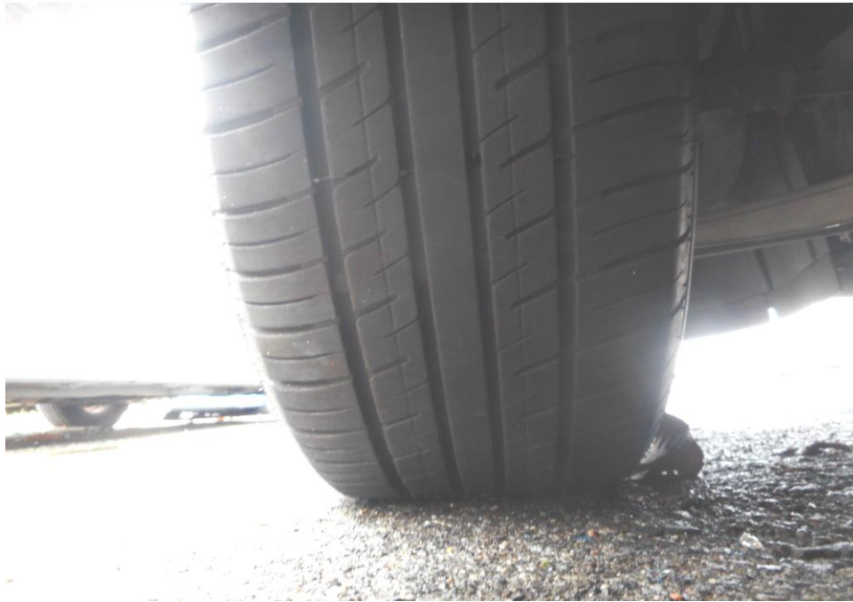
Photo 10 shows the condition of the front left tyre of the Motor Car, which was observed to be in serviceable condition with remaining tread depth of approximately 4.9mm. There was also no tear, cut or burst mark(s) on the outer and the inner sidewalls as well as across the tread of the Motor Car's 4 tyres.
