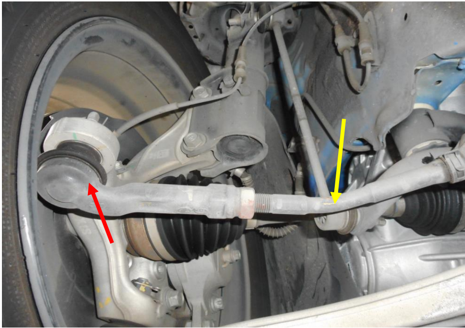
Photo 22 shows the various undercarriage components at the front left wheel of the Motor Car, which had included the steering tie rod (red arrow). The tie rod (yellow arrow) was observed to be damaged a bent as a result of the accident.
