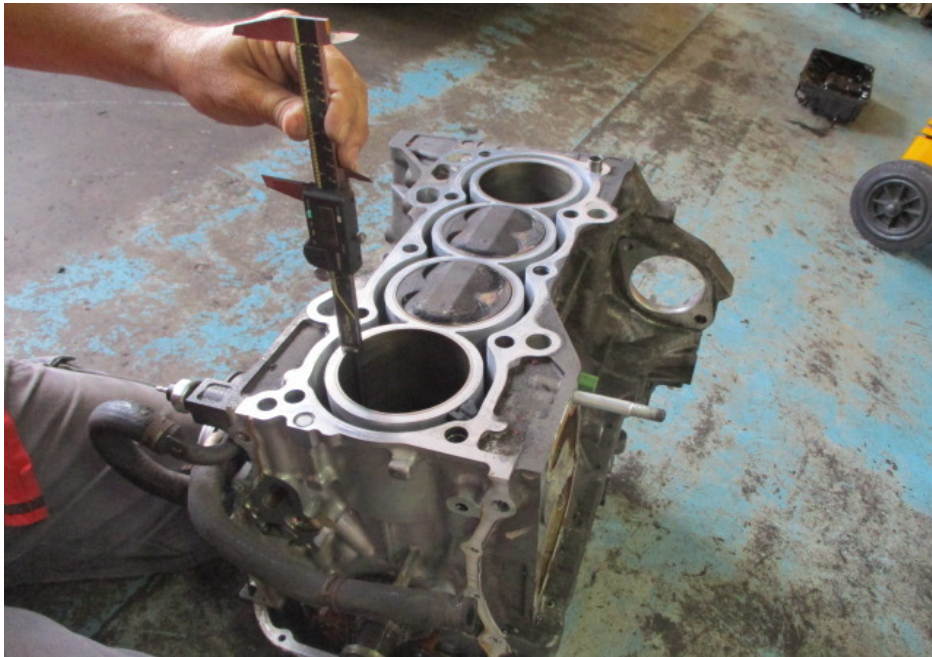
Photo 9 shows measurement being carried out to the stroke of cylinder 1 of the Honda engine. The bore and stroke measurements of the Honda engine were carried out using a digital Vernier Caliper.
