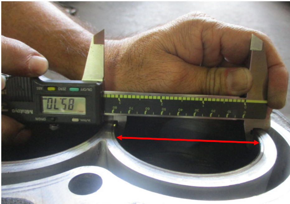
Photo 20 shows the bore measurement of cylinder 4, which was recorded to be 85.70mm.
