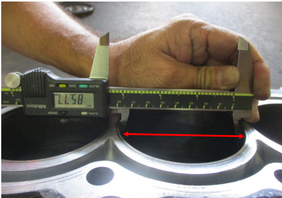
Photo 12 shows measurement being carried out to the bore (arrowed) of cylinder 2 of the Honda engine. The bore measurement of cylinder 2 was recorded to be 85.77mm.
