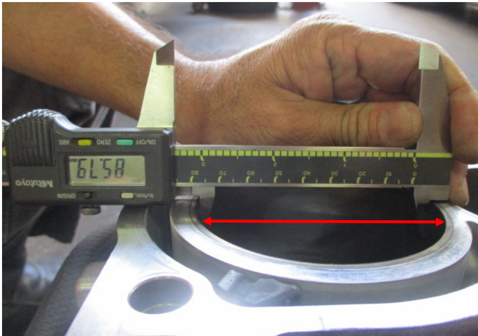
Photo 8 shows the bore measurement of cylinder 1, which was recorded to be 85.79mm.
