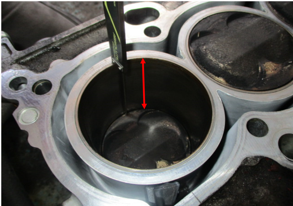
Photo 10 shows measurement being carried out to the stroke (arrowed) of cylinder 1 of the Honda engine. The bore and stroke measurements of the Honda engine were carried out using a digital Vernier Caliper that was calibrated before the start of the measurements,
