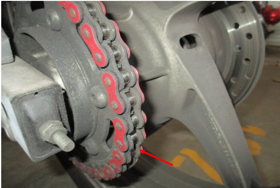
Photo 21 shows a closer view of the gear train (arrowed) of the Motorcycle, which was observed to be intact with no misalignment. It was also adequately lubricated for operating purposes.
