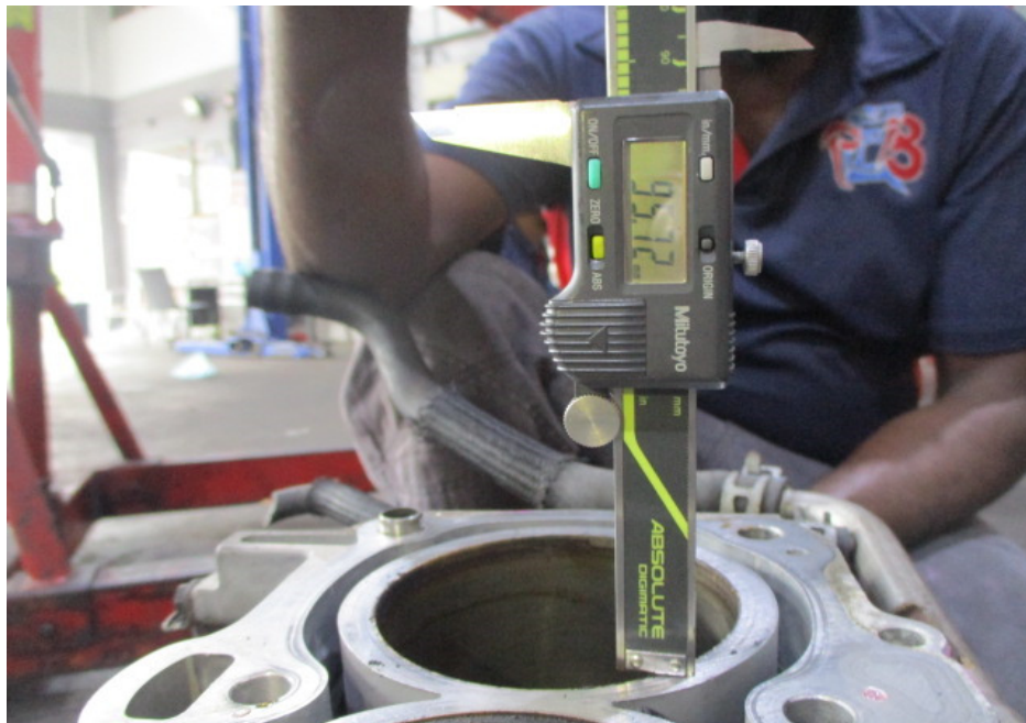
Photo 19 shows the stroke measurement of cylinder 4, which was recorded to be 95.72mm.
