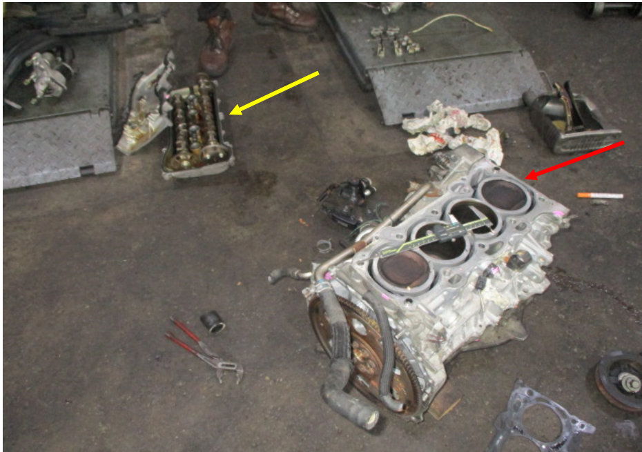
Photo 5 shows the top block (yellow arrow) of the Toyota engine separated from its bottom block (red arrow). This was to enable me to carry out measurements of its cylinders, in particular the bore and stroke measurements of each cylinder, which typically can be used to determine the engine displacement or more commonly referred to as engine cc.
