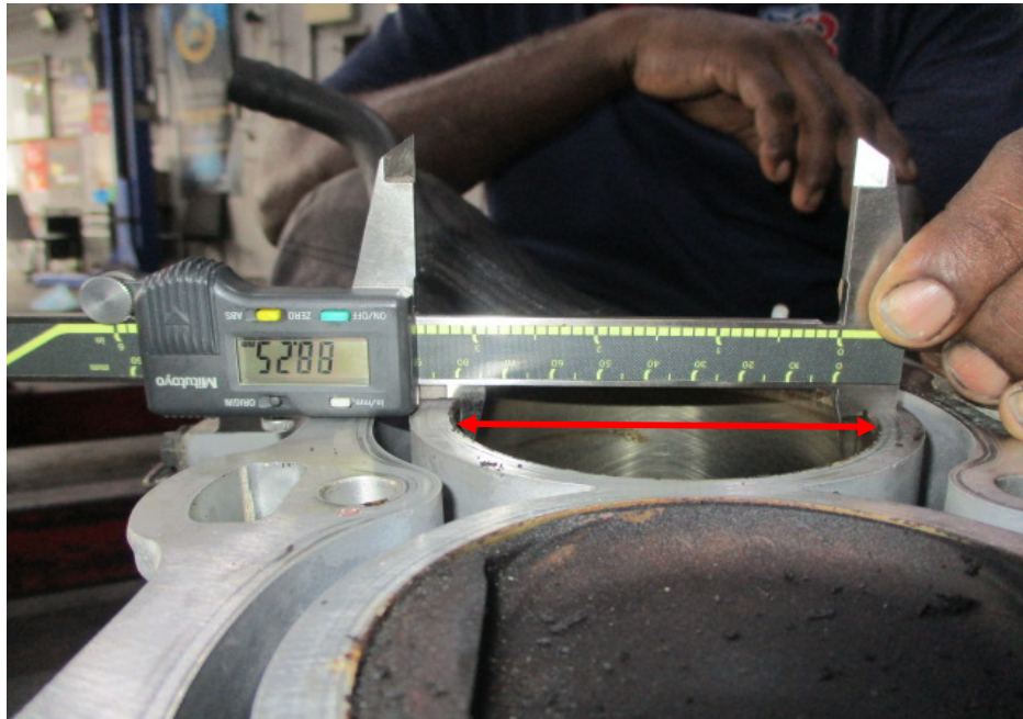
Photo 17 shows measurement being carried out to the bore (arrowed) of cylinder 4 of the Toyota engine. The bore measurement of cylinder 4 was recorded to be 88.25mm.
