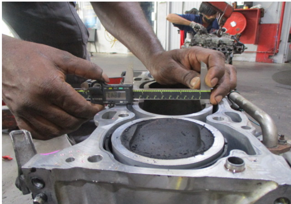
Photo 10 shows measurement of the bore for cylinder 2 of the Toyota engine that I had inspected. The bore and stroke measurements of the Toyota engine were carried out using a digital Vernier Caliper that was calibrated before the start of the measurements.
