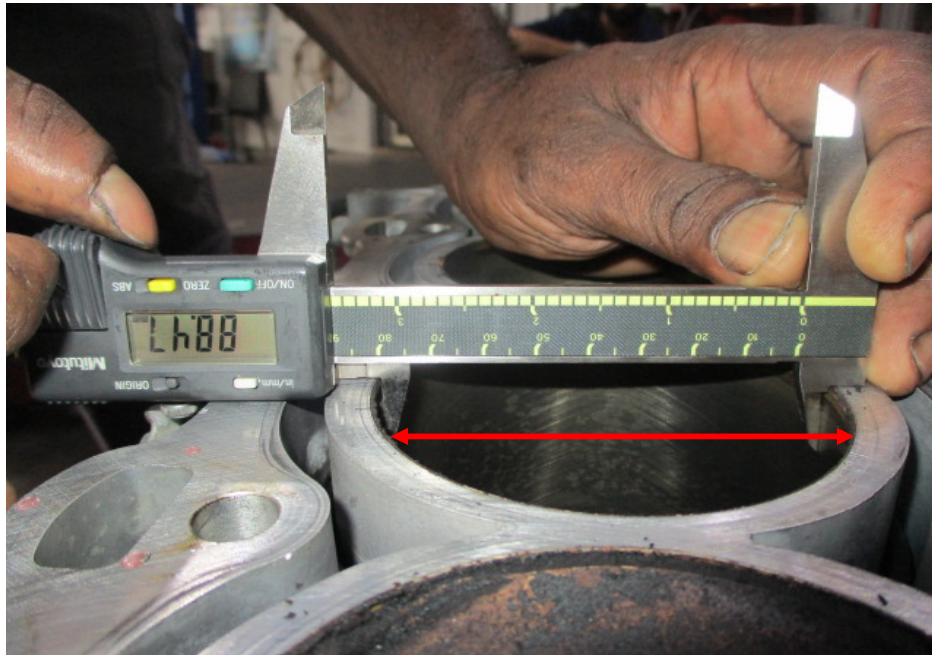
Photo 11 shows measurement being carried out to the bore (arrowed) of cylinder 2 of the Toyota engine. The bore measurement of cylinder 2 was recorded to be 88.47mm.
