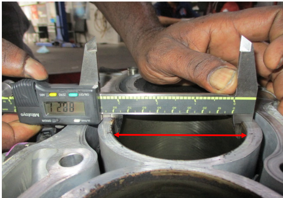
Photo 14 shows measurement being carried out to the bore (arrowed) of cylinder 3 of the Toyota engine. The bore and stroke measurements of the Toyota engine were carried out using a digital Vernier Caliper that was calibrated before the start of measurements. The bore measurement of cylinder 3 was recorded to be 88.21mm.
