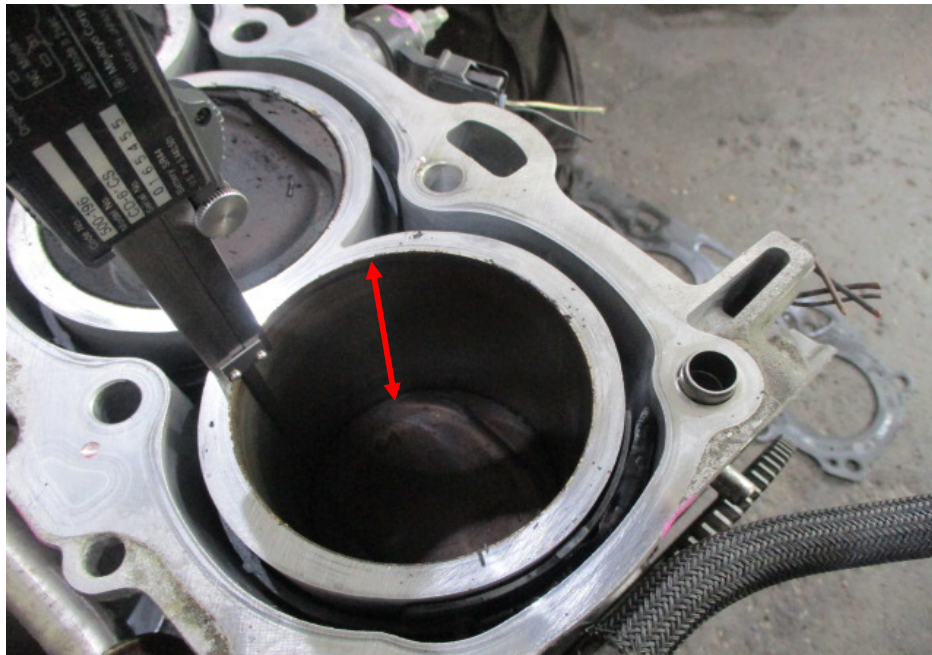
Photo 18 shows measurement being carried out to the stroke (arrowed) of cylinder 4 of the Toyota engine. The bore and stroke measurements of the Toyota engine were carried out using a digital Vernier Caliper that was calibrated prior to the start of measurements.
