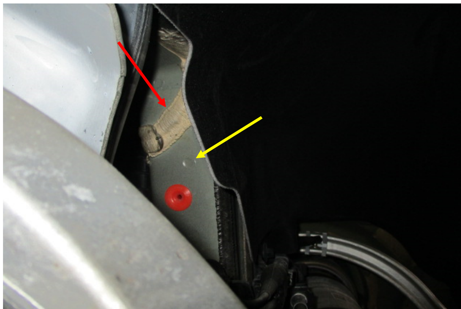
Photo 20 shows the chassis/structural body at the underside front left of the Motor Car. I did not find any weld marks other than original spot weld marks (yellow arrow) on the chassis/structural body of the Motor Car. The original factory sealant (red arrow) at the joints along the chassis/structural body was untouched, indicating no work was done on the chassis/structural body of the Motor Car and that the chassis/structural body was originally fitted.
