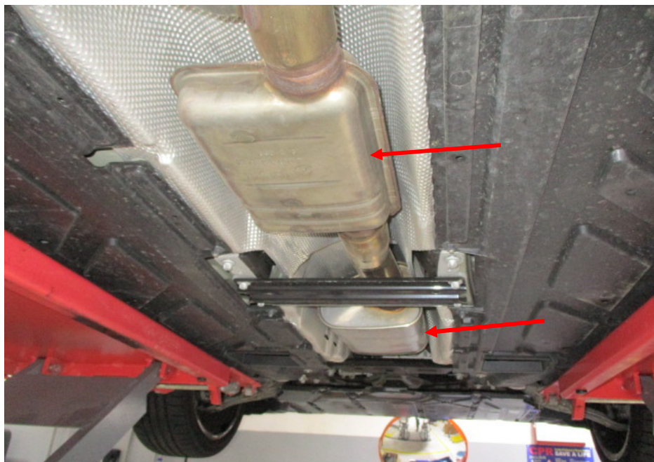
Photo 18 shows the Motor Car's centre resonators (arrowed). My examination of the Motor Car's exhaust system revealed no sign(s) or indication(s) of any cut or weld marks along its exhaust pipes and on its catalytic convertor.
