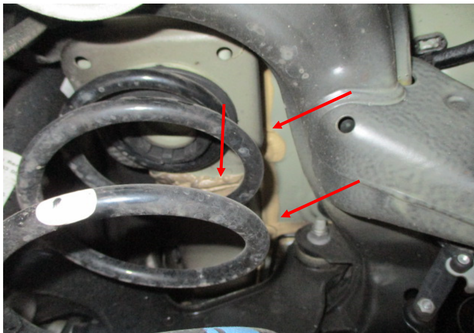
Photo 20 shows the chassis/structural body at the underside rear left of the Motor Car. Visually, The original factory sealant (arrowed) at the joints along the chassis/structural body was untouched, indicating no work was done on the chassis/structural body of the Motor Car and that the chassis/structural body was originally fitted.
