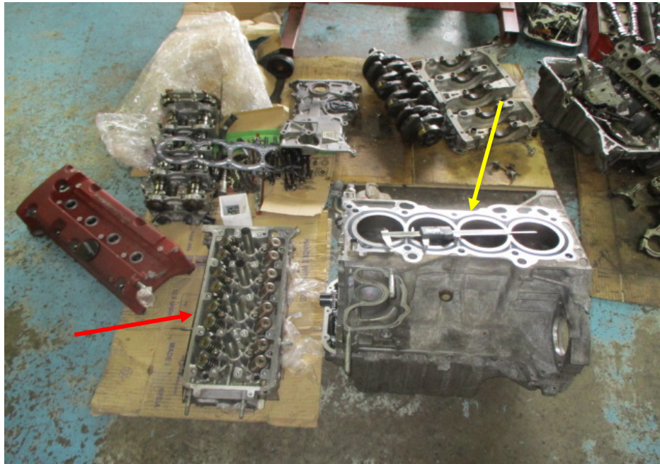
Photo 5 shows the top block (red arrow) of the Honda engine separated from its bottom block (yellow arrow). This was to enable me to carry out measurements of its cylinders, in particular the bore and stroke measurements of each cylinder, which typically can be used to determine the engine displacement or more commonly referred to as engine cc.
