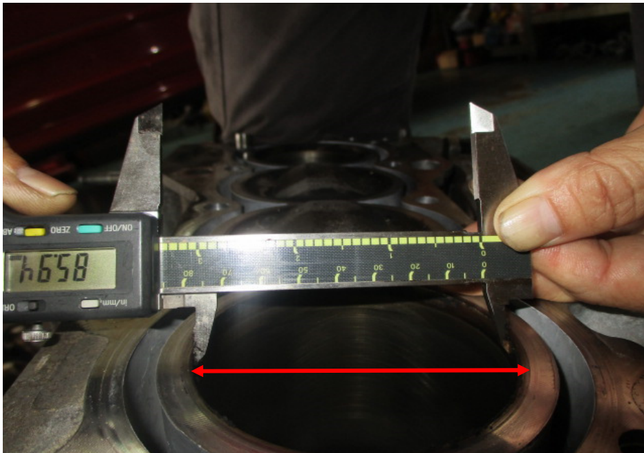
Photo 20 shows the bore measurement of cylinder 4, which was recorded to be 85.94mm.
