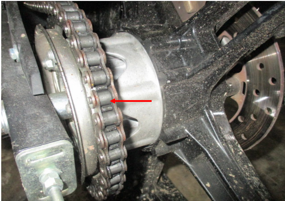
Photo 17 shows a closer view of the gear train (arrowed) of the Motorcycle, which was observed to be intact with no misalignment. It was also adequately lubricated for operating purposes.
