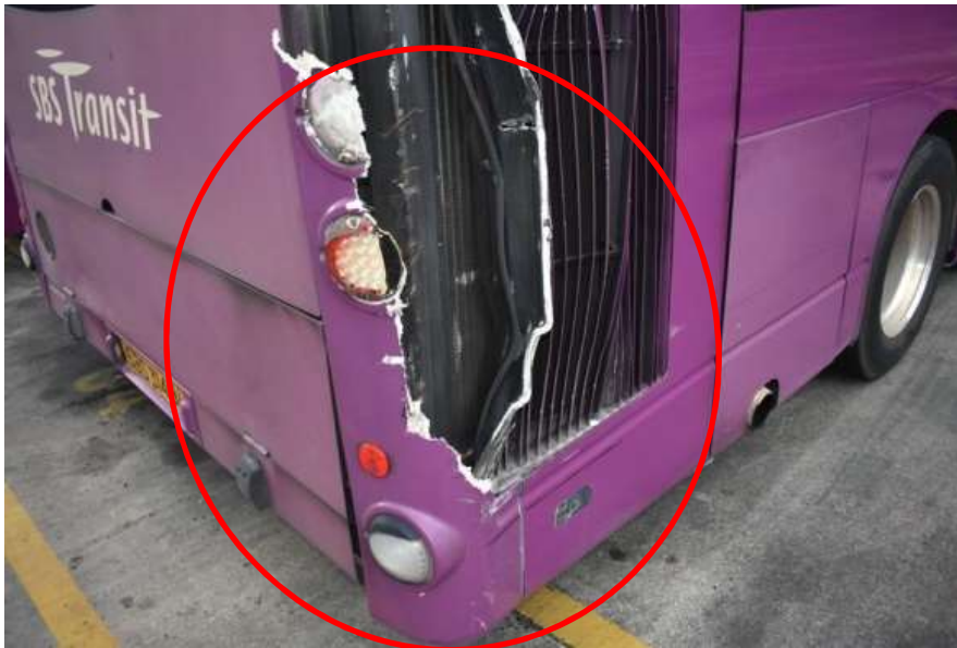
Rear reverse lamp assembly, dislodge/damaged
