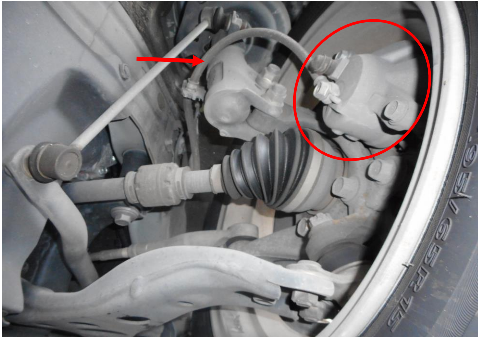
Photo 18 shows the brake hose/pipe (arrowed) at the front left wheel of the Motor Taxi. No leakage of brake fluid was observed. Visual examination of the various components of the braking system like the brake caliper (circled), brake booster, brake pedal etc had revealed all to be intact and without visible damage.
