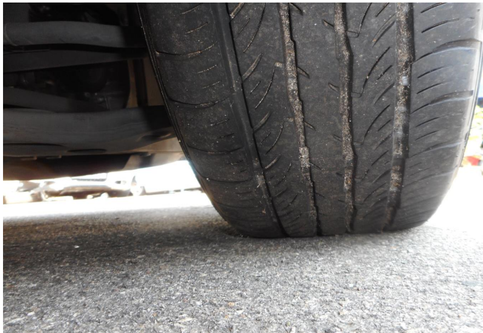
Photo 5 shows the condition of the front right tyre of the Motor Taxi, which was observed to be in serviceable condition with remaining tread depth of approximately 4mm. The tyre was sufficiently inflated for vehicular operation with no tear, cut or burst mark(s) on the outer and the inner sidewalls as well as across the tread. The 4 tyres of the Motor Taxi were wrapped around standard alloy wheel rims without any damage.
