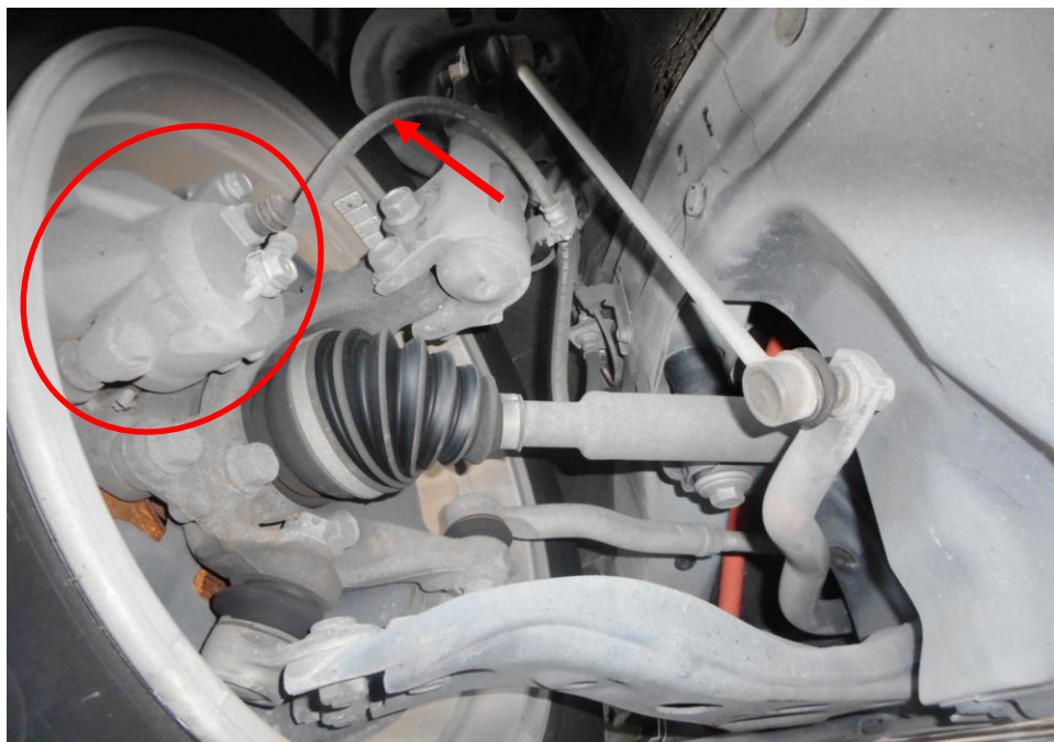
Photo 17 shows the brake hose/pipe (arrowed) at the front right wheel of the Motor Taxi. No leakage of brake fluid was observed. Visual examination of the various components of the braking system like the brake caliper (circled), brake booster, brake pedal etc had revealed all to be intact and without visible damage.
