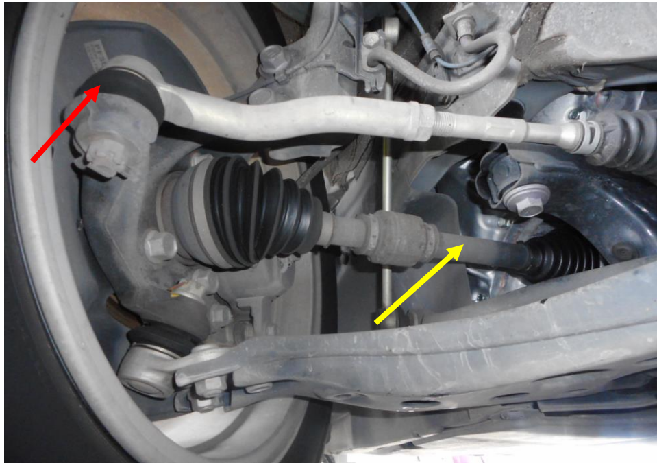
Photo 20 shows the various undercarriage components at the front left wheel of the Motor Taxi, which had included the steering tie rod (red arrow) and front left drive shaft (yellow arrow). The various undercarriage components of the Motor Taxi were all found to be intact without any visible damage.
