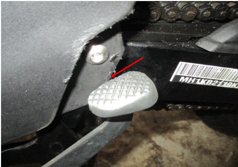
Photo 9 shows as a result of the accident, the rear portion of the gear shift pedal was bent inwards, causing it to be stuck to the lower portion of the left subframe of the Motorcycle (arrowed).
