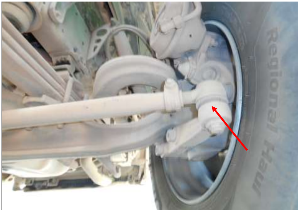
Photo 21 shows the various undercarriage components at the front right wheel of the Motor Lorry, in particular the steering tie rod end (arrowed). The various steering components were all found to be intact, suggesting that the steering system of the Motor Lorry was likely to be in serviceable condition at the material time of accident. There was also no sign of fluid stain(s) observed on the various undercarriage components.
