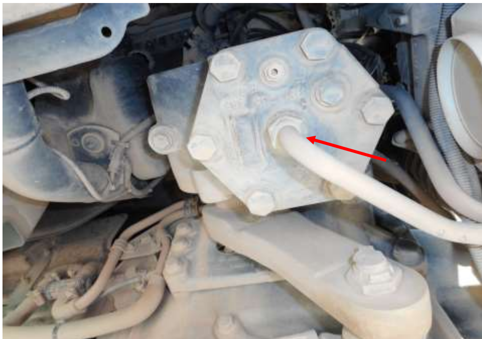
Photo 23 shows the steering box component (arrowed) at the undercarriage of the Motor Lorry was found to be intact without any visible damage. There was also no sign of fluid stain(s) observed on the various undercarriage components.
