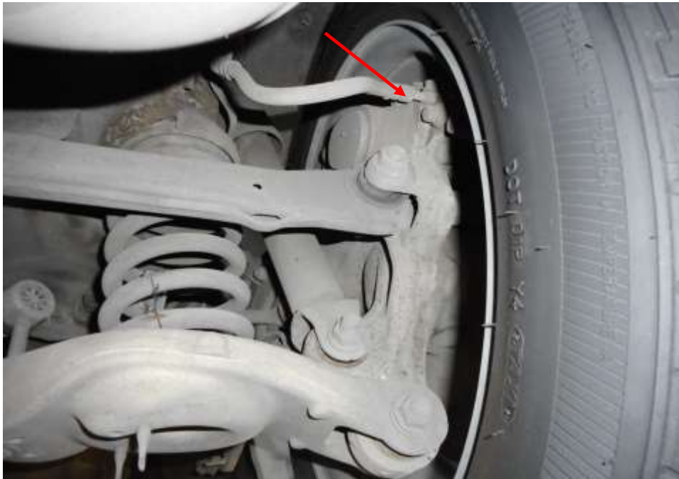
Photo 18 shows the brake hose/pipe (arrowed) at the rear right wheel of the Motor Taxi. No leakage of brake fluid was observed. Visual examination of the various components of the braking system like the drum brake, brake booster, brake pedal etc had revealed all to be intact and without visible damage.
