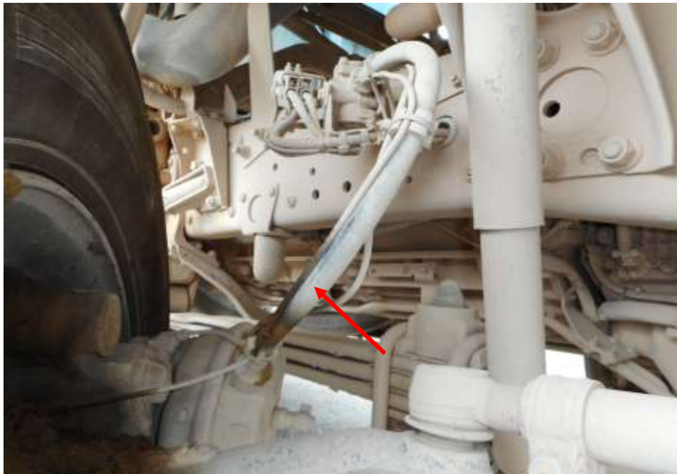
Photo 19 shows the brake pipe (arrowed) at the front right wheel of the Tipper Lorry. I did not observe any leakage of brake fluid at the time of my inspection of the Tipper Lorry. My static tests of the Tipper Lorry's braking system, along with my visual examination of the various mechanical components in the braking system had indicated that there was no internal leakage of pressure/vacuum. Hence the braking system of the Tipper Lorry was likely to be in serviceable condition at the material time of accident.
