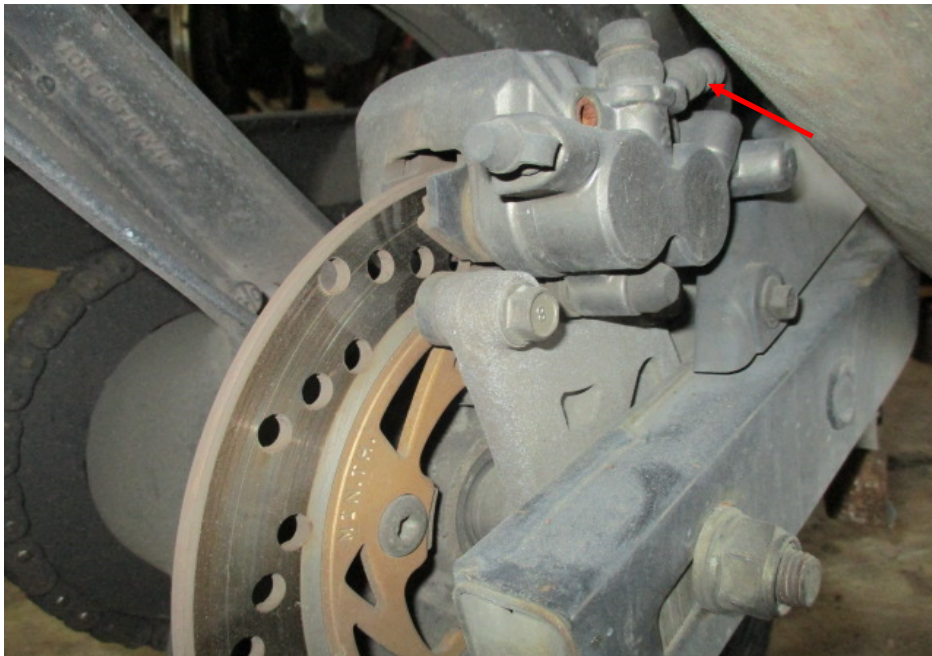
Photo 20 shows a close up view of the rear brake caliper, rear brake disc and rear brake hose (arrowed) of the Motorcycle, which are all part of the components in the hydraulic rear brake system of the Motorcycle. Our visual checks of these various components had revealed all to be intact with no visible damage. No leakage of brake fluid was also observed.
