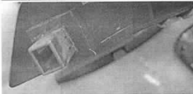
45/66: Repairer's Photo
