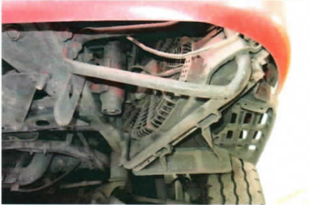
29/32: Inspection Photo
