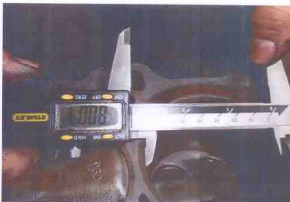
Photo 10 shows the bore measurement of cylinder 2, which was recorded to be 80.07mm.
