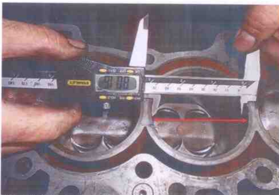
Photo 13 shows measurement being carried out to the bore (arrowed) of cylinder 3 of the Honda engine. The bore and stroke measurements of the Honda engine were carried out using a digital Vernier Caliper. The bore measurement of cylinder 3 was recorded to be 80.16mm.
