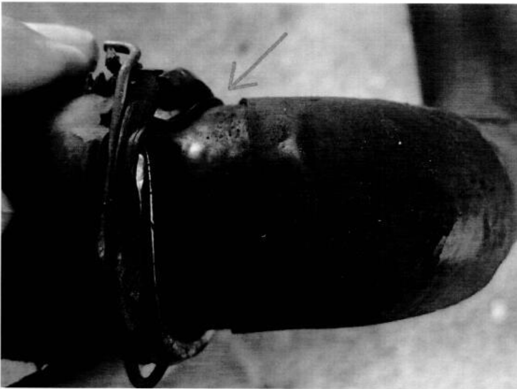
Radiator top hose LH – torn
