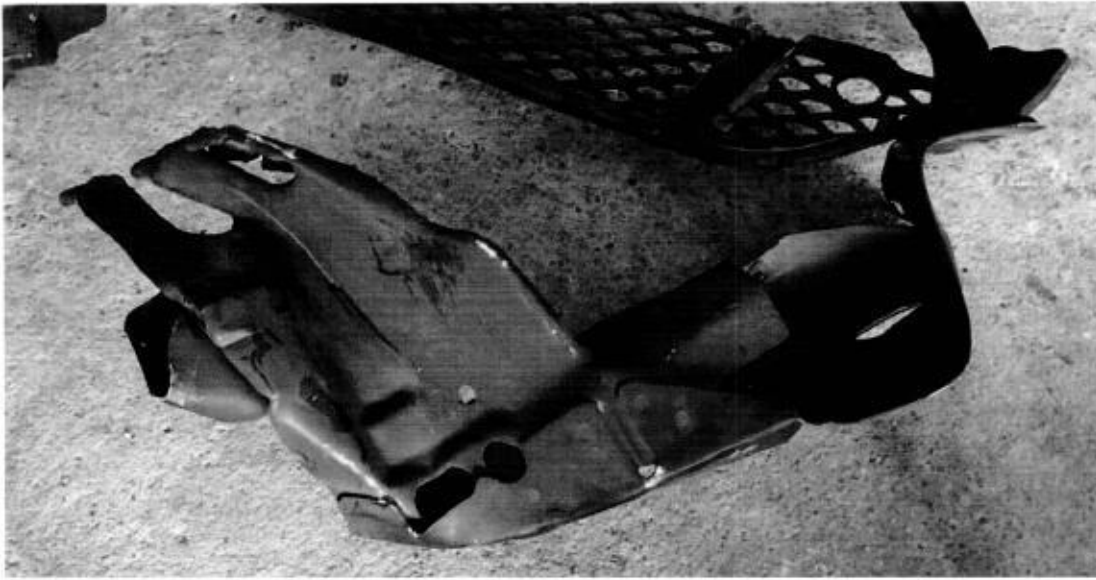
Headlamp panel bracket - bent
